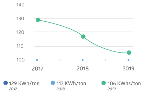
OLC | Electricity KWh/ton
